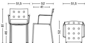
BALCONY DINING ARMCHAIR Width 51,5 cm Depth 52 cm Height 81 cm Seat height 46 cm Seat depth 41 cm
