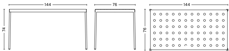
BALCONY TABLE Length 144 cm Width 76 cm Heigth 74 cm
