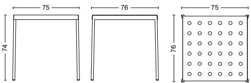
BALCONY TABLE Length 75 cm Width 76 cm Heigth 74 cm
