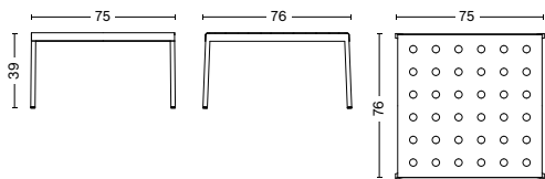
BALCONY LOW TABLE | SQUARE Length 75 cm Width 76 cm Heigth 39 cm
