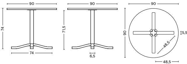
PASTIS TABLE Diameter 90 cm Height 74 cm Weight 15,6 kg
