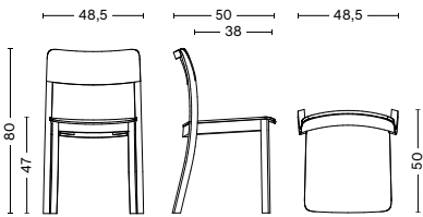
PASTIS CHAIR Width 48,5 cm Depth 50 cm Height 80 cm Seat height 47 cm Seat depth 38 cm Weight 6 kg
