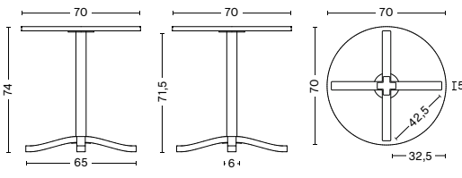
PASTIS TABLE Diameter 70 cm Height 74 cm Weight 9 kg
